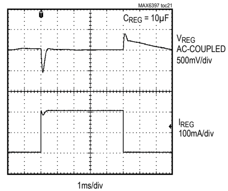
REG LOAD-TRANSIENT RESPONSE
